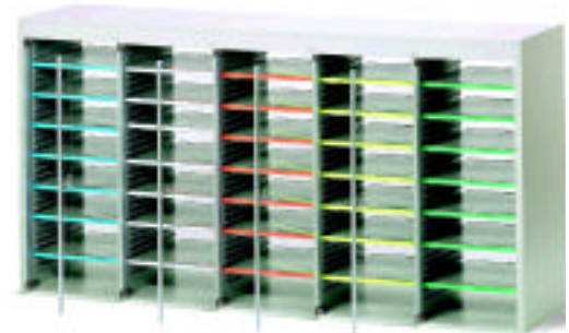
Five section wide Sort Module with open back and transparent doors.
